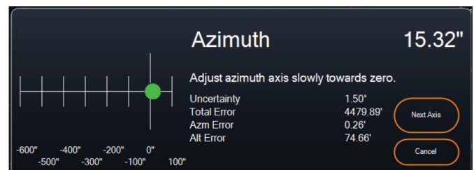
Fig. 18: Azimuth Axis Adjustment window during polar alignment in CPWI.
